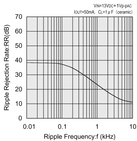
XC6202PC02 (12V)
